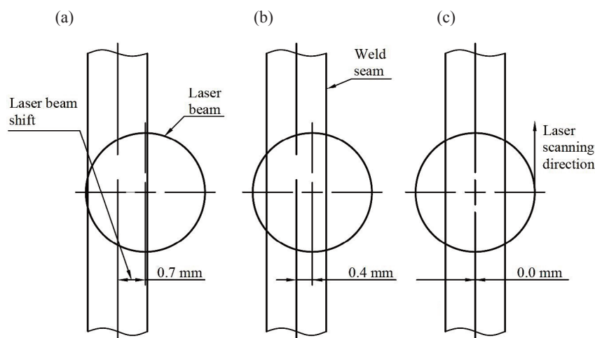
Fig. 3. Schematic presentation of laser beam irradiation from the centre of the weld in the laser absorbent part at the following shifts: (a) 0.7 mm; (b) 0.4 mm and (c) 0.0 mm.
