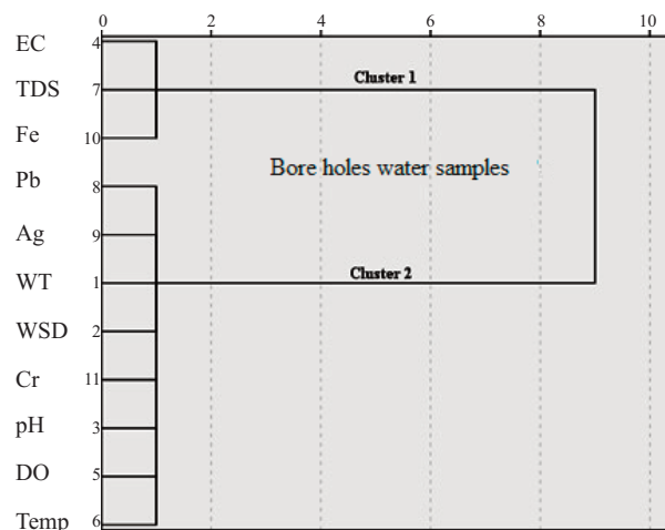
Fig. 5. HCA dendrogram (using Ward Linkage) of BH water parameters.
