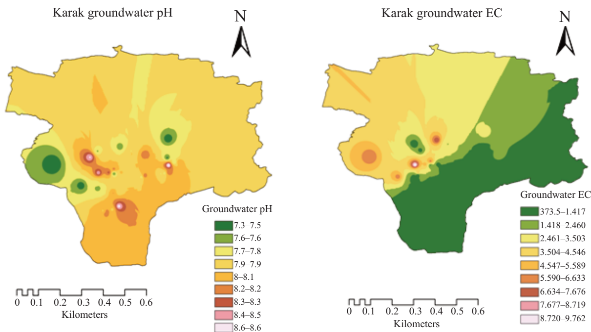
Fig. 3. The pH content and electrical conductivity (EC) of groundwater in \mu\text{S}/\text{cm} in different locations.
