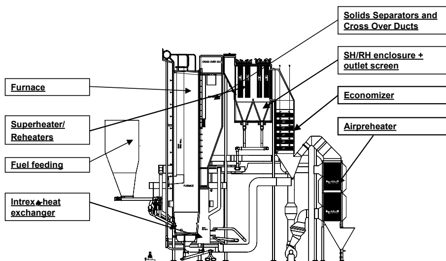
Fig. 2. Boiler concept for Estonian oil shale
