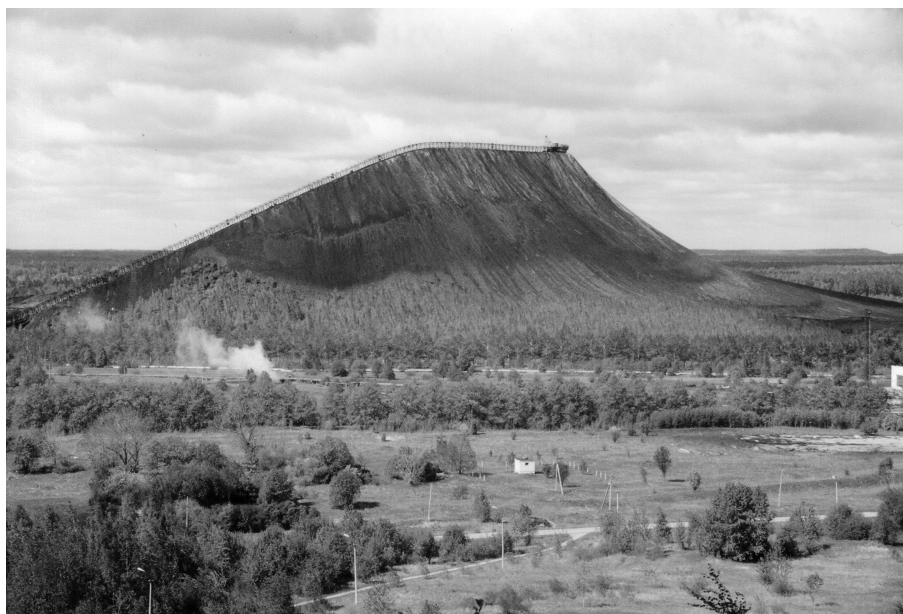
Fig. 2. New semi-coke mountain near the town of Kiviõli (relative height 116 m) (author of the photo: Riina Vaht)
