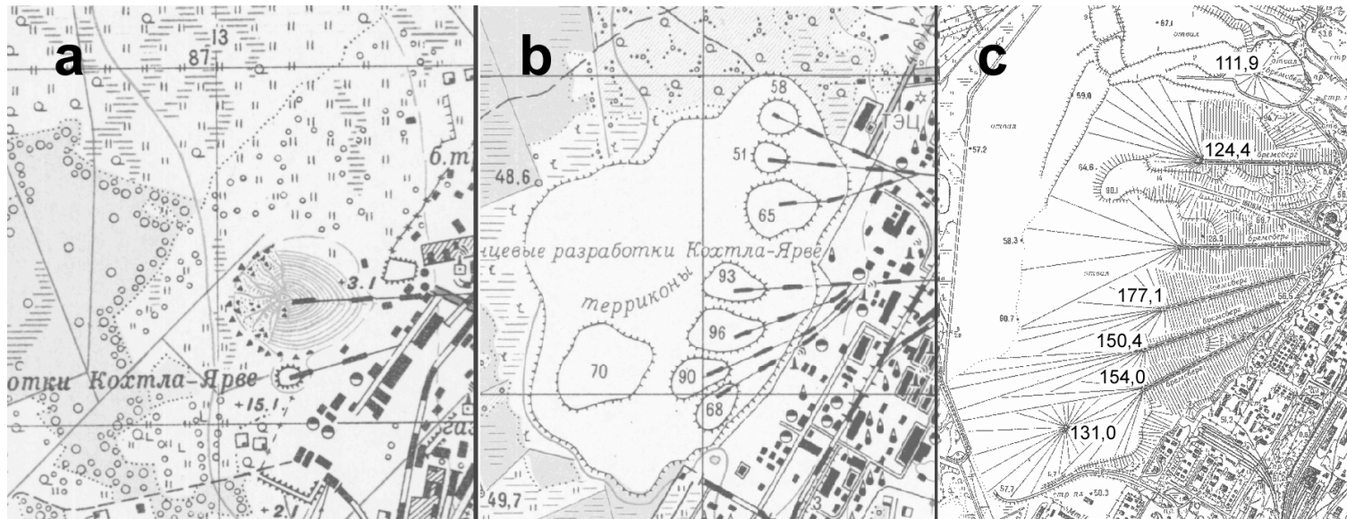
Fig. 4. The development of Kohtla-Järve semi-coke mountains in the maps from different periods: a –1947, b –1960, c –1980
